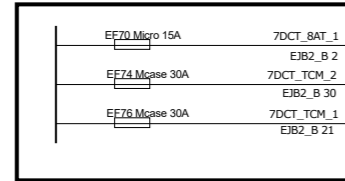
15/49 ENGINE JUNCTION BOX EJB2 B:8889694516
