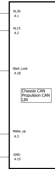
4/209 TRANSMISSION ACTUATOR CONTROL MODULE TACM A:8889623993
