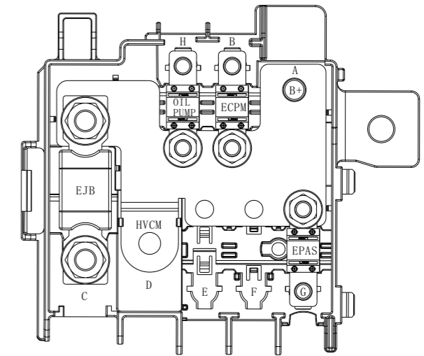
3. Fuse arrangement HMDB
