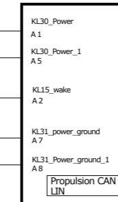
4/209 TRANSMISSION ACTUATOR CONTROL MODULE TACM A:8889623993
